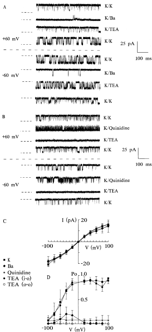
Fig. 4. Effect of blockers on \text{K}^+ channel activity. (A) Representative recordings showing the reversible ability of \text{Ba}^{2+} to reduce the open probability and the lack of effect of TEA on a single inside-out patch at a holding potential of \pm 60 mV (filtered at 3 kHz). Pipet and bath solutions were symmetric 140 mM KCl with either 5 mM \text{Ba}^{2+} or 5 mM TEA added to the bath solution (internal surface). (B) Representative recordings of a single channel from an outside-out patch at a holding potential of \pm 60 mV (filtered at 3 kHz). Note that quinidine produced a flickery block and TEA completely blocked channel activity. Pipet and bath solutions were symmetric 140 mM KCl with either 5 mM quinidine or 5 mM TEA added to the bath solution (external surface). (C) Current-voltage relationship over a range of holding potentials for inside-out patches showing that the current amplitude was not affected by the addition of 5 mM \text{Ba}^{2+} ( \blacklozenge ), 5 mM quinidine ( * ) or 5 mM TEA ( \bullet ) to the bathing solution containing 140 mM KCl with 140 mM KCl in the pipet. Data are means \pm s.d. for 5–8 experiments. (D) Open probability of \text{K}^+ channels over a range of holding potentials for inside-out (closed symbols) i.e. internal surface and outside-out (open symbols) i.e. external surface, patches in the presence of 5 mM \text{Ba}^{2+} ( \blacklozenge ), 5 mM quinidine ( * ) or 5 mM TEA ( \bullet and \circ ) to the bath solution containing 140 mM KCl with 140 mM KCl in the pipet. Data are means \pm s.d. for 5–8 experiments.
